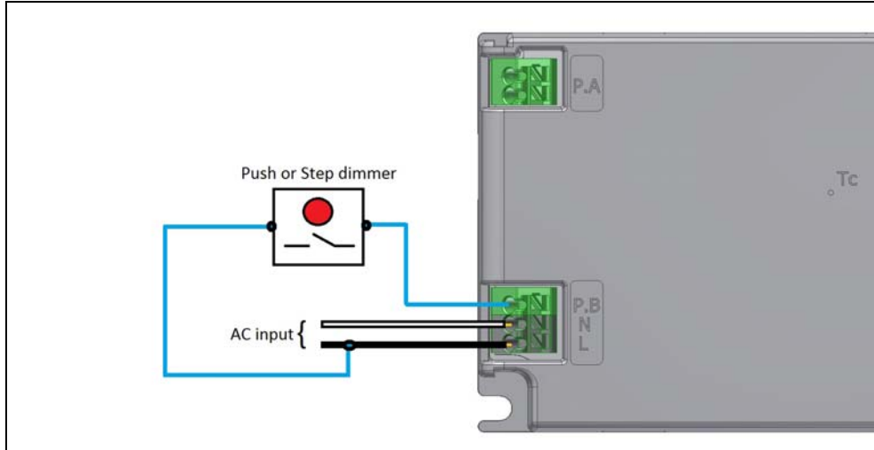
Figure 9: Connection of a Push or Step dimmer.
