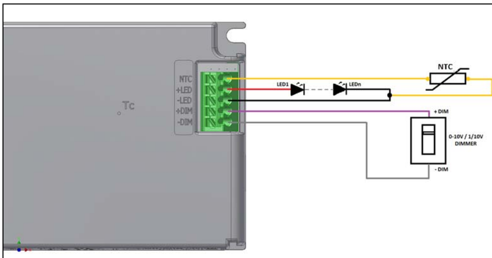
Figure 8: Connection of a 0-10/1-10V dimmer and NTC.
