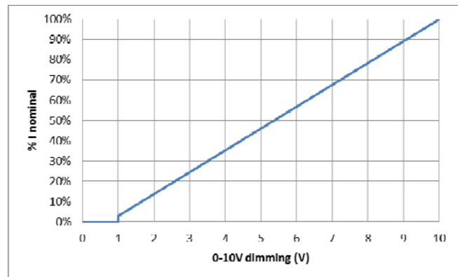
Figure 7: Output Current (%) along dimming input voltage for 0-10V option
